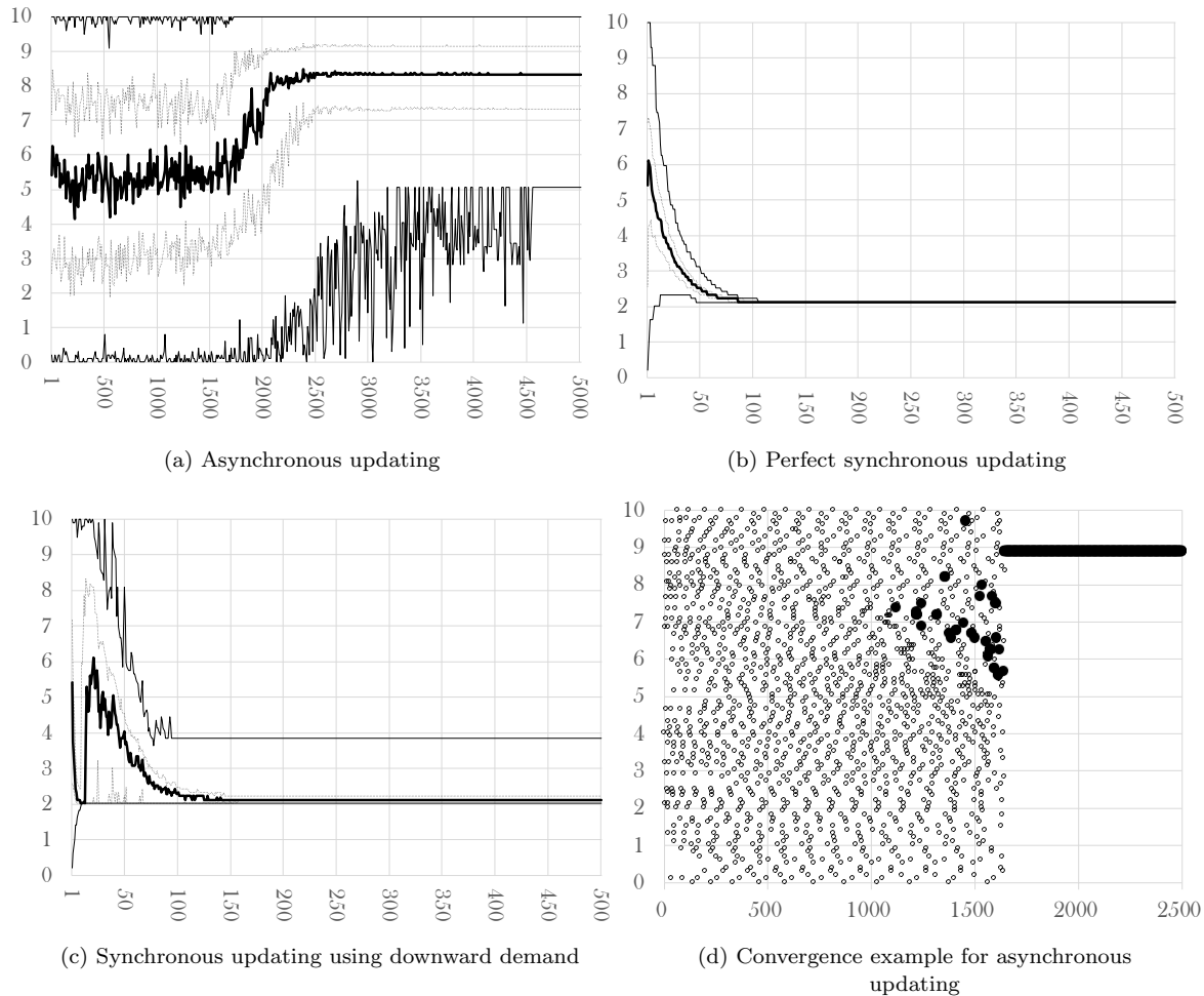
Figure 1. : Price outcomes with different algorithm designs
